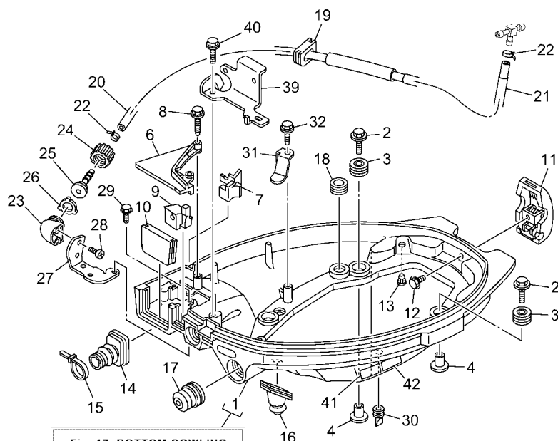
Fig. 17, BOTTOM COWLING Ref. No. 8, 32, 40 Fig. 13, ELECTRICAL 1 Ref. No. 26, 38 Fig. 21, CONTROL 2 Ref. No. 33
